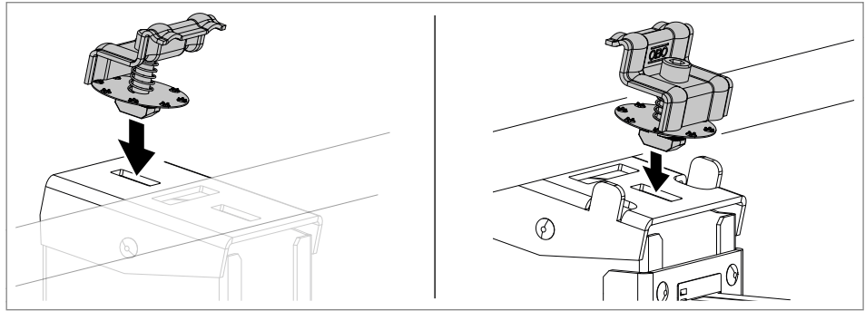
Fig. 32: Inserting end clamps with springs in slots
